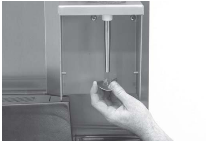
Figure 23. Removing Agitator From Shaft
