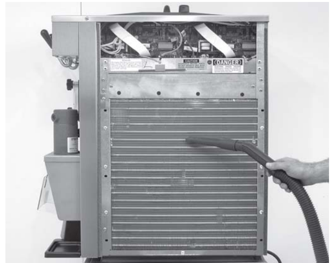
Figure 30. Cleaning Condenser
